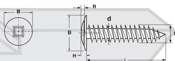
Square Recess
