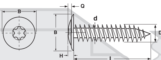
Six-Lobe Recess
