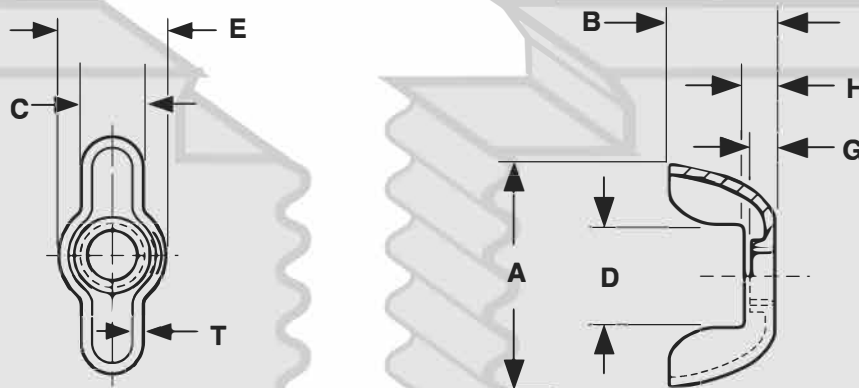
WING NUTS - STAMPED (TYPE-D)
