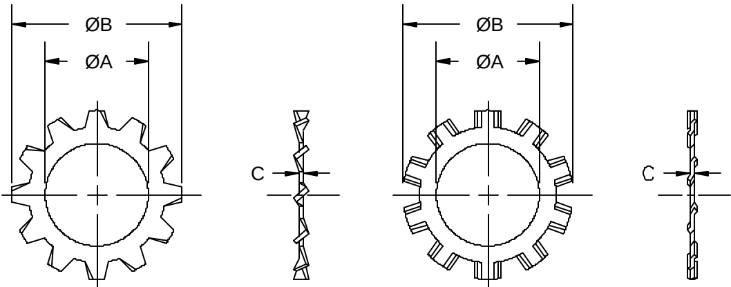
ACCEPTABLE DESIGNS Figure 1. Lock washer.
