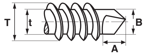
5/16 & 3/8 Diameter #3 Point
